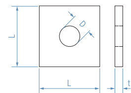
Bearing plate
