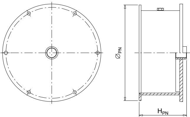
Protection cap N
