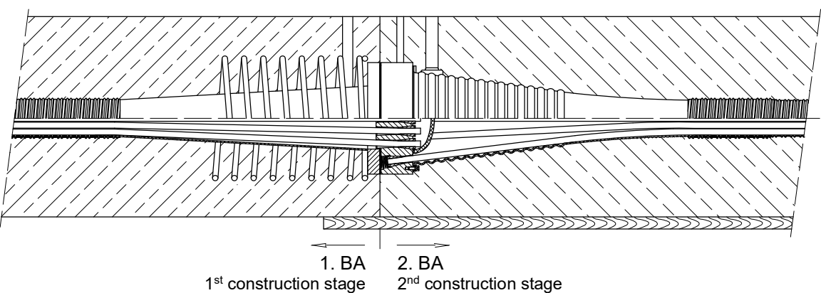
Fixed and stressing coupler FK, SK
