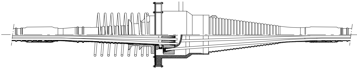
Electrically isolated fixed and stressing coupler FKE, SKE 1)
