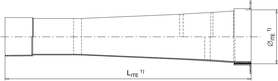
Plastic trumpet A SP 0206–3106
