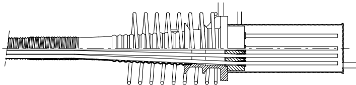
Restressable / exchangeable anchorage with monostrands or grease / wax, SAR 1)
