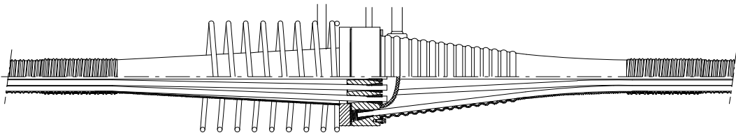
Fixed and stressing coupler FH, SH
