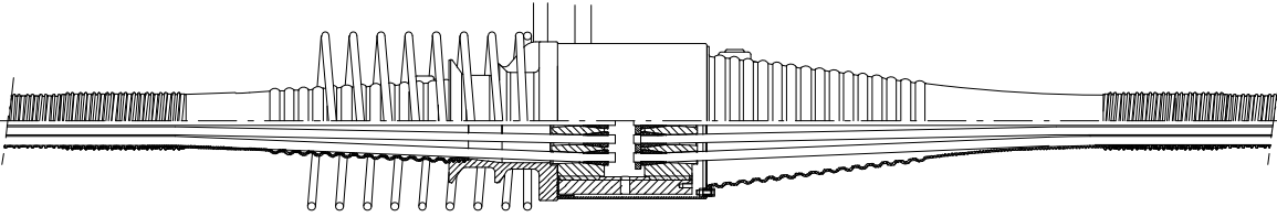
Fixed and stressing coupler FH, SH 1)
