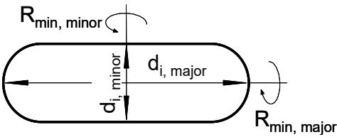
Inner dimensions, d_i , of flat duct and minimum radius of curvature, R_{min}
