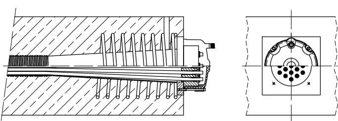
Exposed stressing anchorage SA
