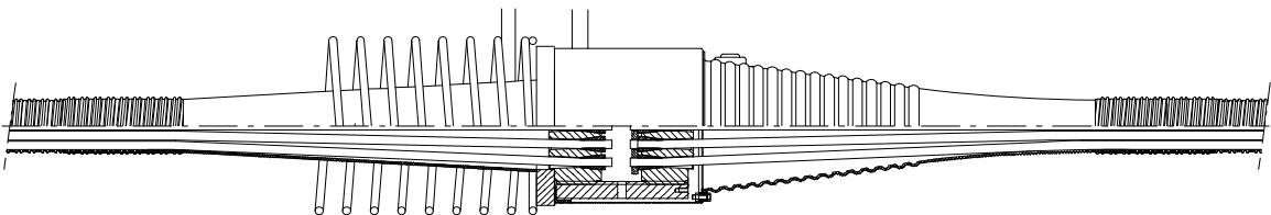
Restressable / exchangeable anchorage
