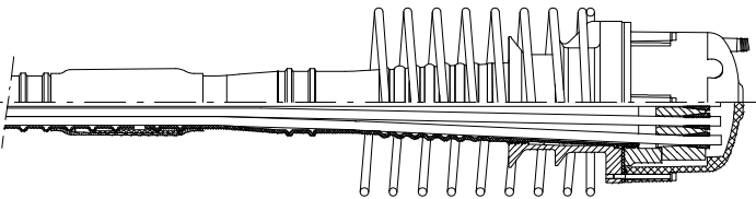
Electrically isolated stressing, electrically isolated accessible fixed anchorage SAE, FAE 1)
