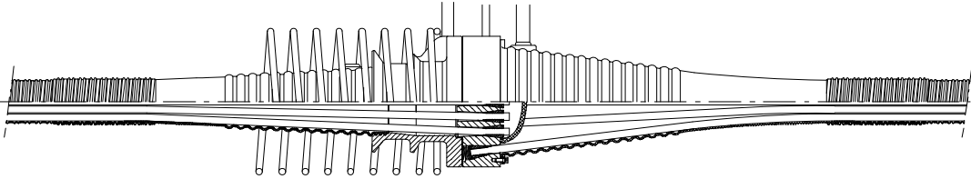
Fixed and stressing coupler FK, SK 1)
