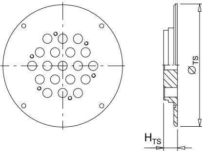
Cover Plate K
