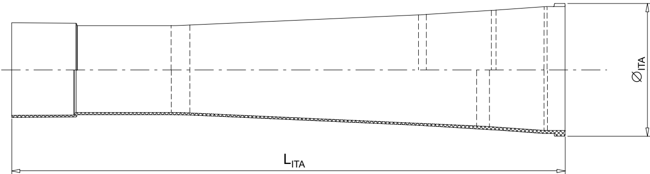
Inner trumpet A
