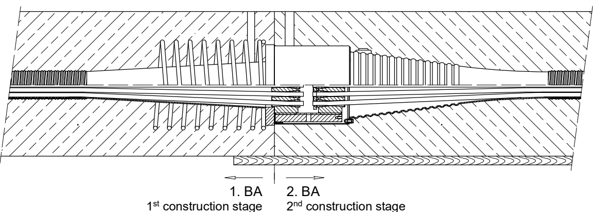
Fixed and stressing coupler FH, SH
