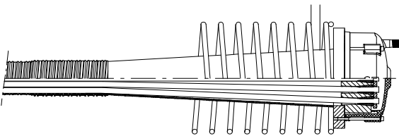
Fixed and stressing coupler FK, SK
