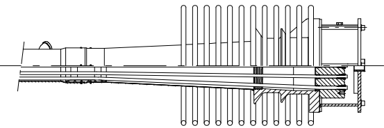
Stressing anchorage nuclear, accessible fixed anchorage nuclear SAN, FAN
