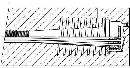
Fixed anchorage FA
