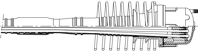
Electrically isolated inaccessible fixed anchorage FAE 1)
