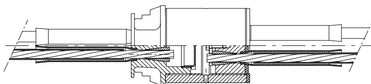
Sleeve coupler H CONA CMM S1-0406 (four)
